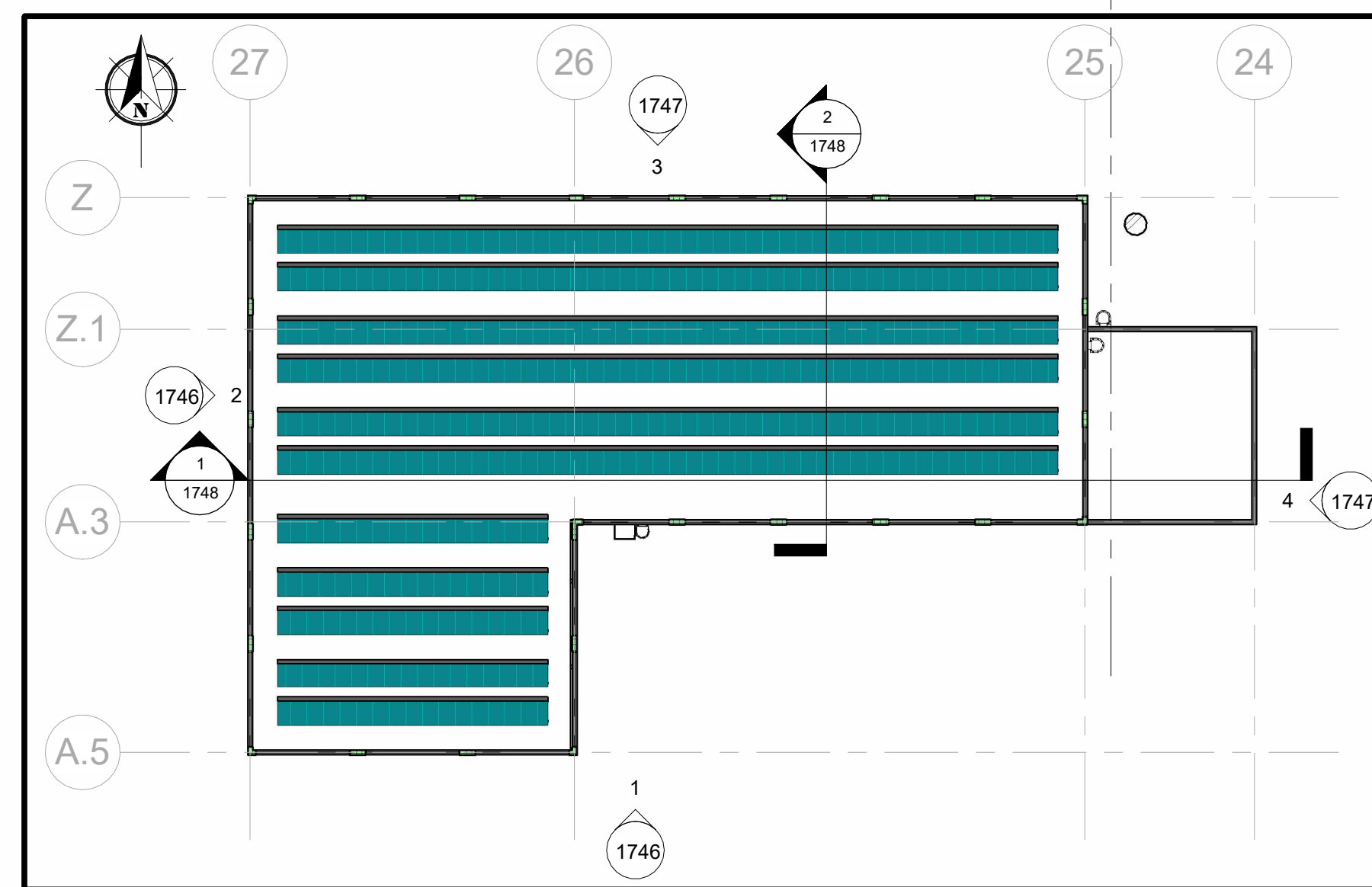
KEYPLAN Scale 1 : 350
